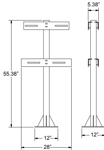
Back-to-back mounting
