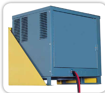
Mounted CWB with charger
